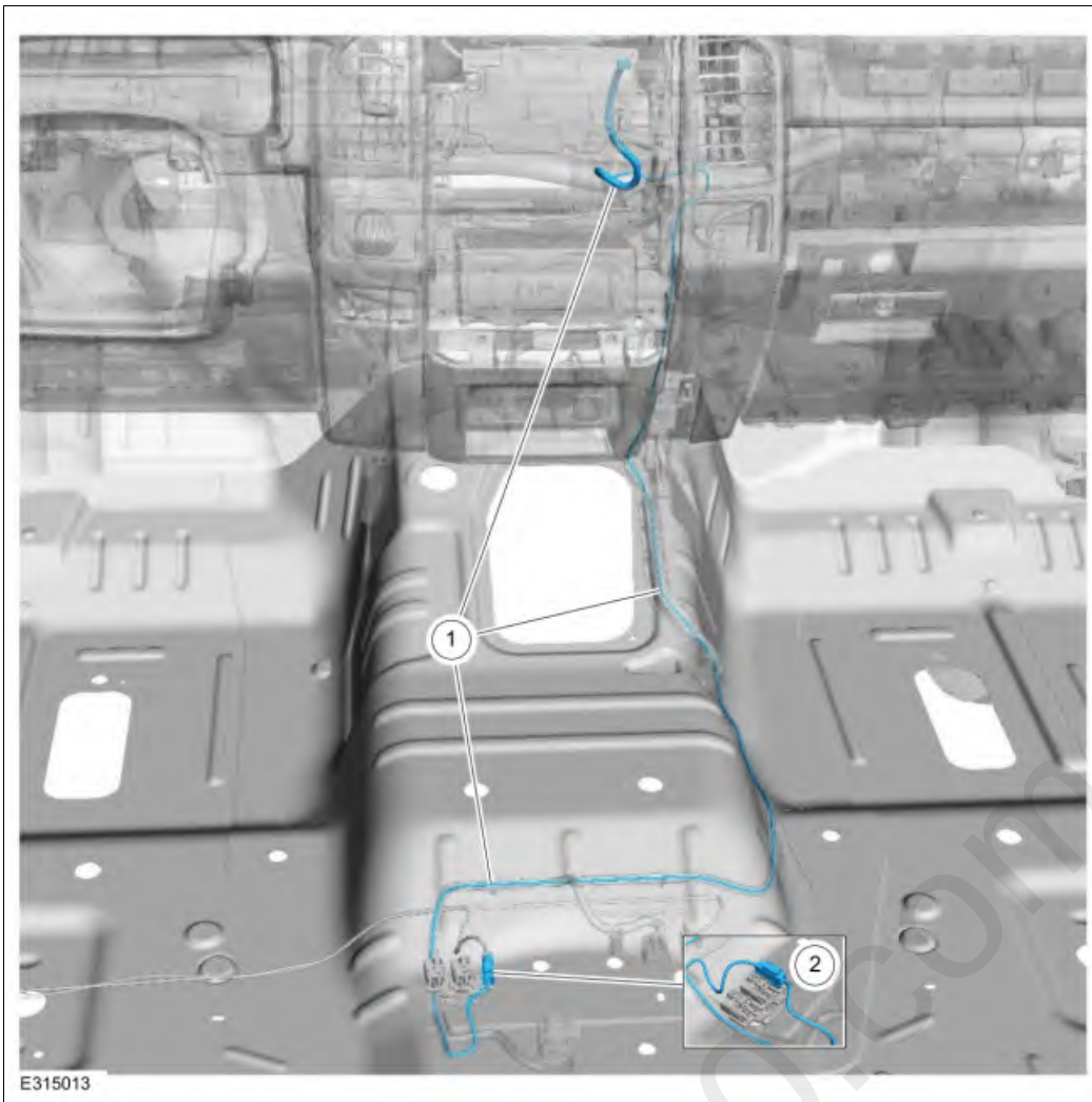
Rear GPS/Satellite Radio Antenna Cable Routing
